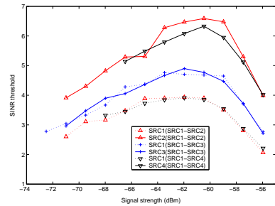
Figure 4: SINR_{\theta} change
